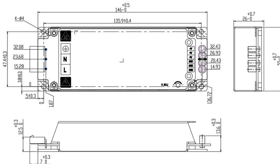
Dimension and mounting hole -- terminal coordinate drawing
